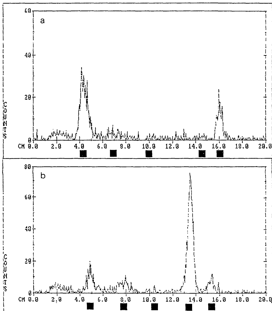
Fig. 2. Radiochromatograms of non-saponifiable lipids extracted from cells of S. cerevisiae incubated with [ ^{14} C]acetate for 2 h. (a) Cells incubated without inhibitors. (b) Cells exposed to 5 \mu M isomer E (compound 1) during the incubation time. The markers from left to right were: ergosterol, lanosterol, dioxidosqualene, oxidosqualene and squalene.
